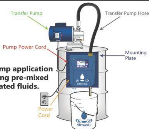
AF-360: Venturi Mixing application for mixing and dispensing water soluble fluids.
