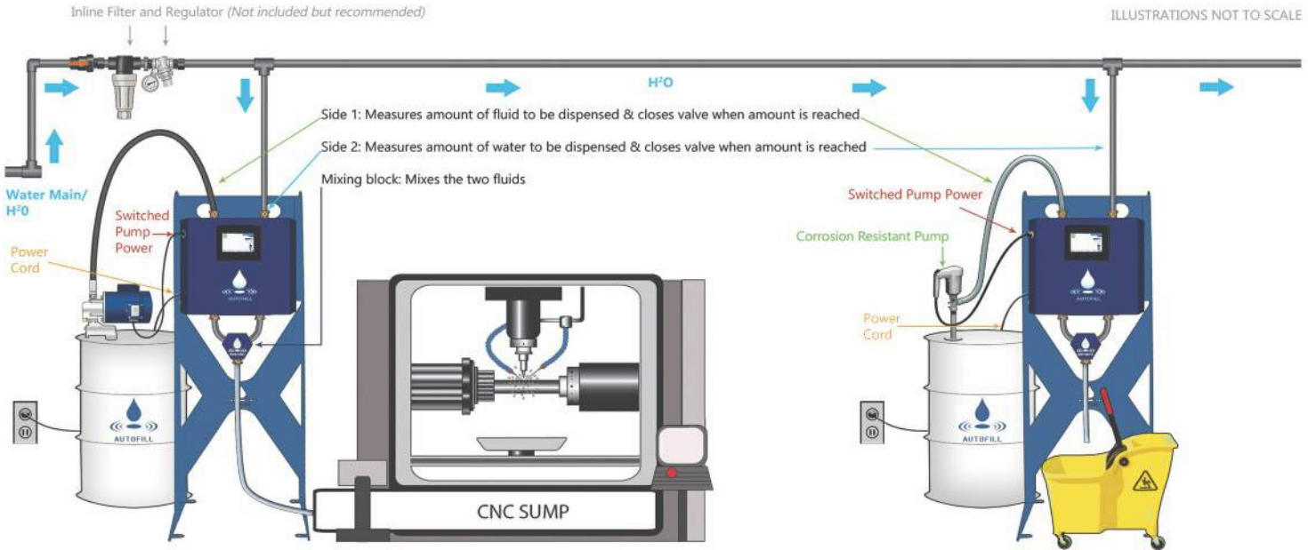
AF-4: Shown with oil pump to mix cutting oil with water and supply CNC machine with mixed cutting fluid.
